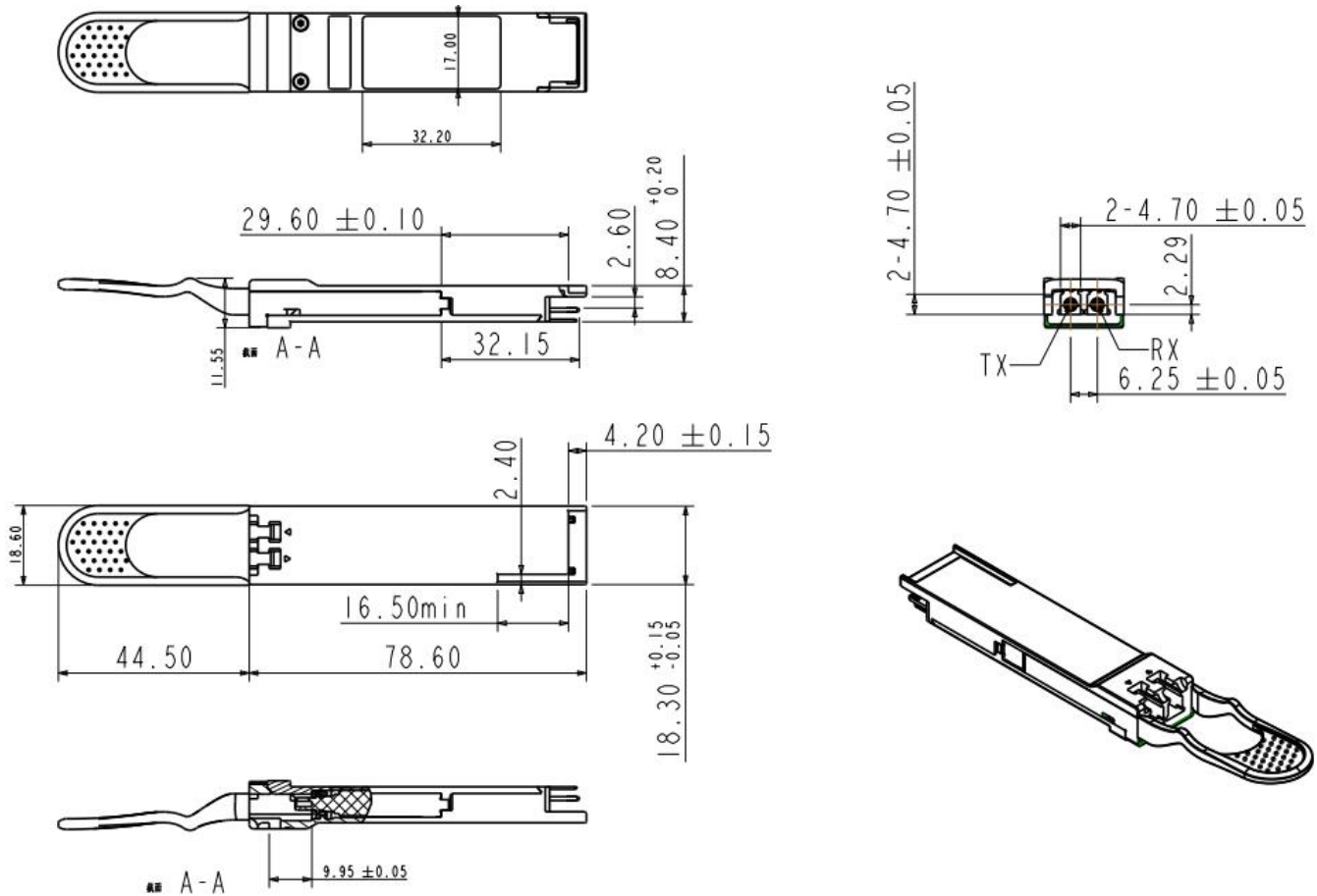
Figure 9 . Mechanical Specifications
